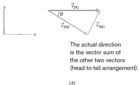
Fig. 4-20 A plane flying in a wind.
